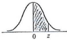
Normal Probabilities
